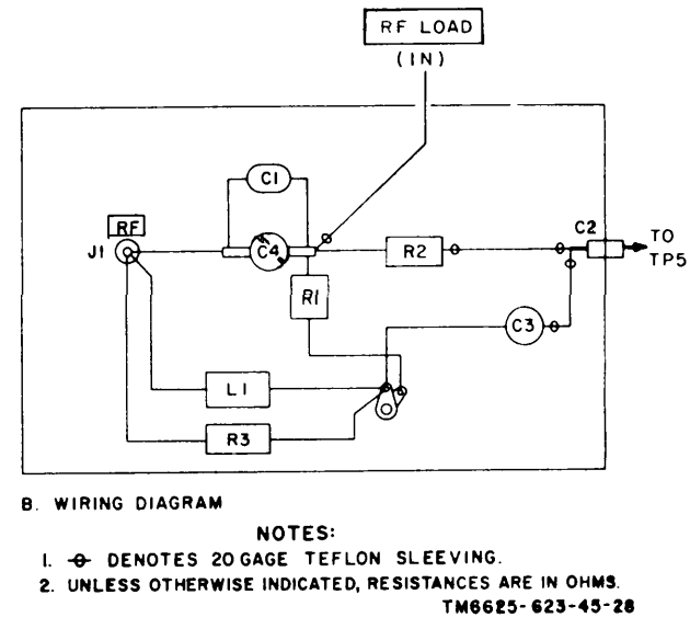
Figure 4-8. If translator dummy load, schematic and wiring diagram.
