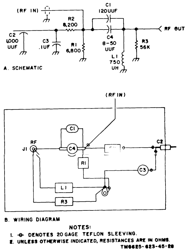
Figure 4-8. If translator dummy load, schematic and wiring diagram.
